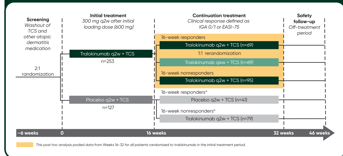
Figure 1. Study design
